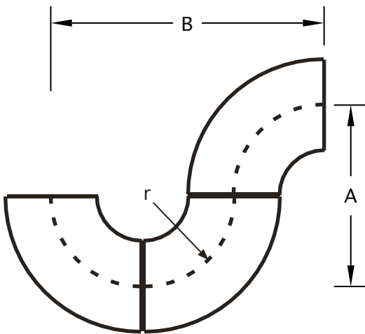
Short Radius P-Trap
