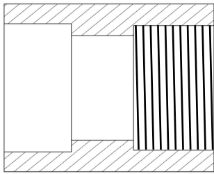
Socket weld x Female NPT
