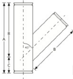
Roll grooved 45° Lateral
