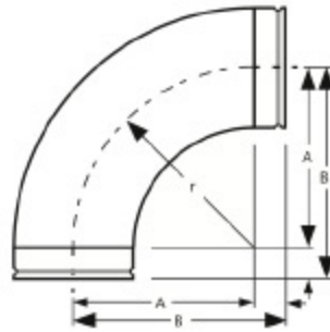
Roll grooved LR90, long tangent
