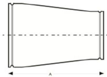
Roll grooved long tangent conc B16.1
