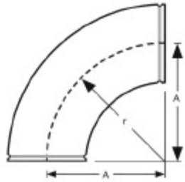
Roll grooved LR90 (no tangents)
